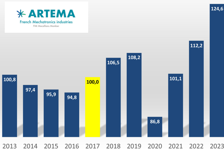
FRENCH MARKET HYDRAULICS 2013-2023 INDEX 100 : 2017
